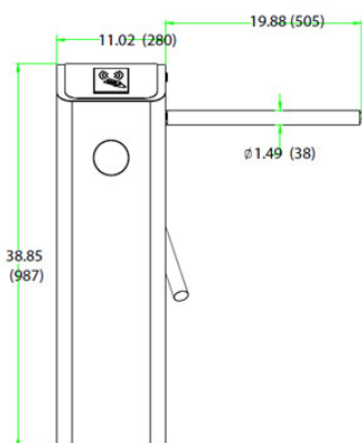
TS2000
